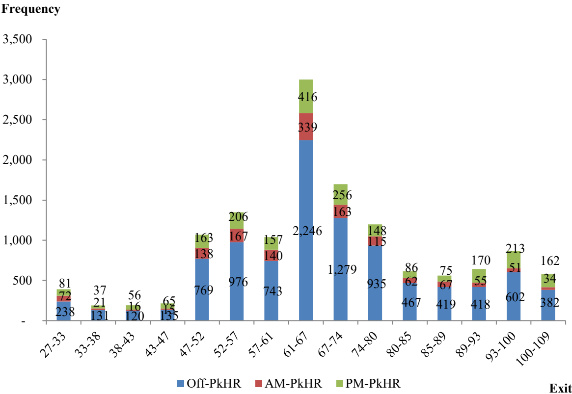
Figure A.2 Distributions of Disabled Vehicles by Time of Day on I-95 in Year 2025
