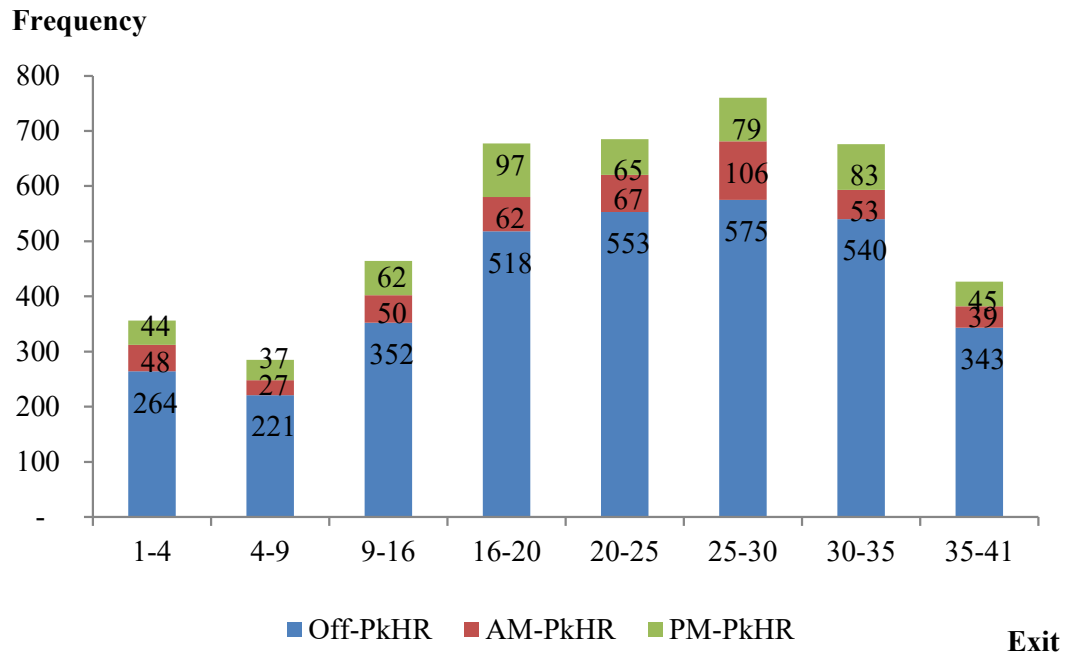
Figure A.3 Distributions of Incidents by Time of Day on I-495 in Year 2025
