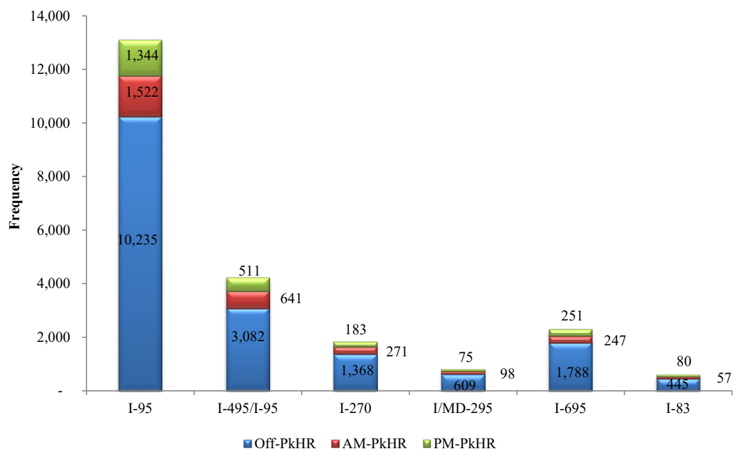
Figure 3.5 Distribution of Disabled Vehicles by Time of Day on Major Roads in 2025
