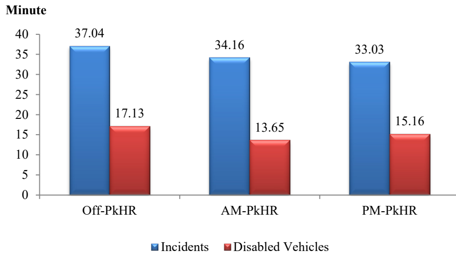
Figure A.11 Distributions of Incident Duration by Time of Day on I-95 in Year 2025
