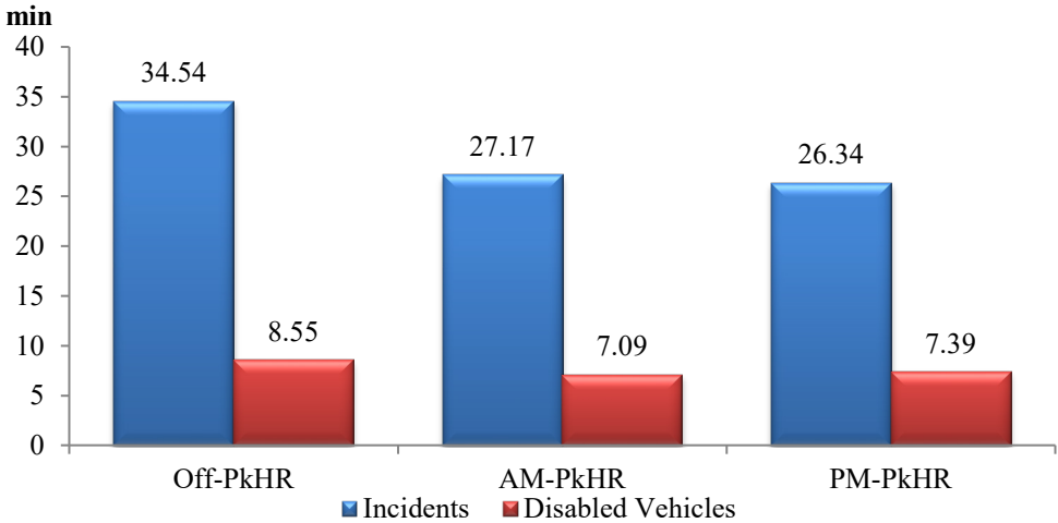
Figure A.10 Distributions of Incident Duration by Time of Day in Year 2025
