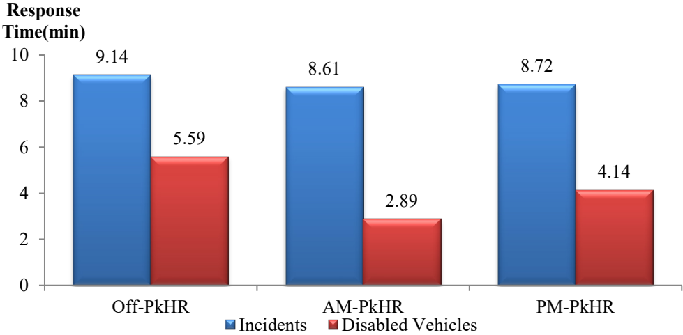
Figure A.9 Distributions of Clearance Time by Time of Day in Year 2025
