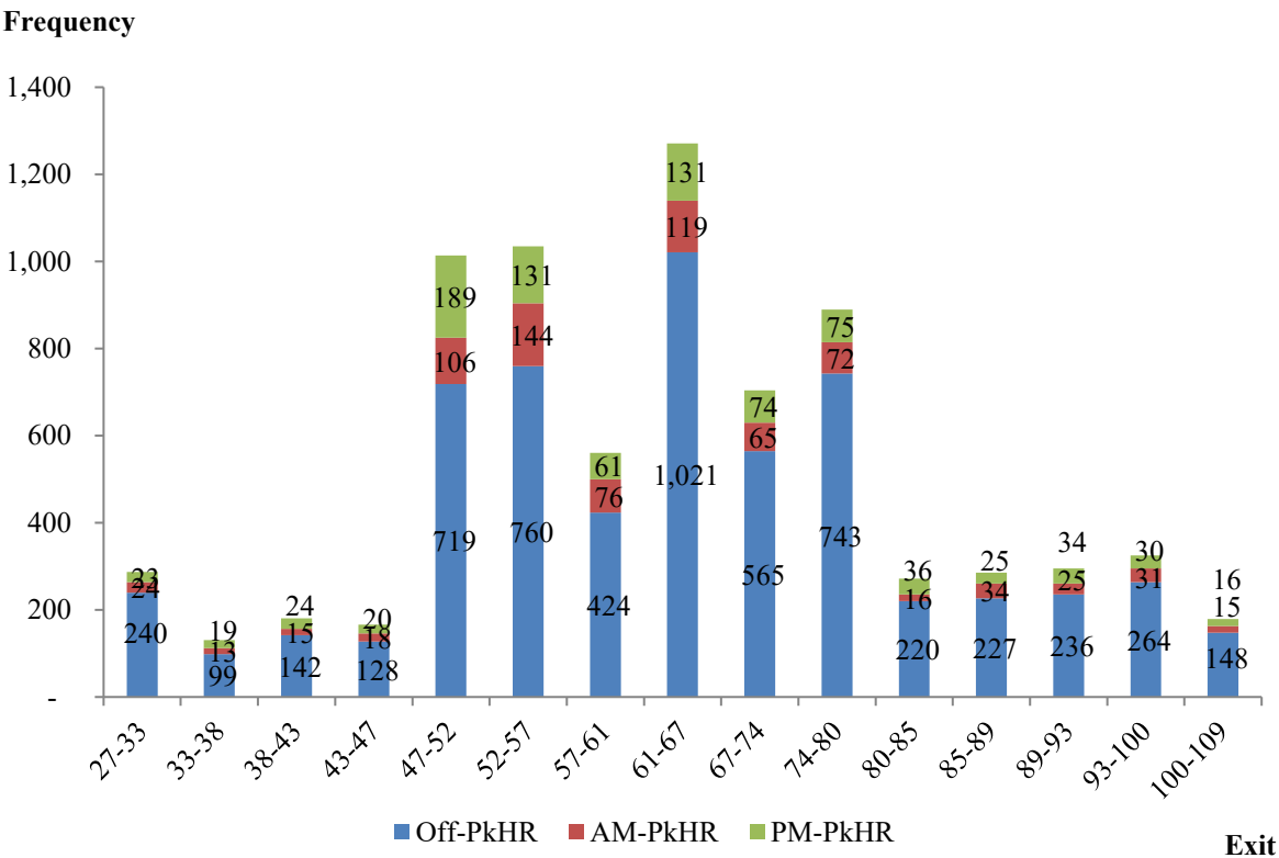
Figure A.1 Distributions of Incidents by Time of Day on I-95 in Year 2025
