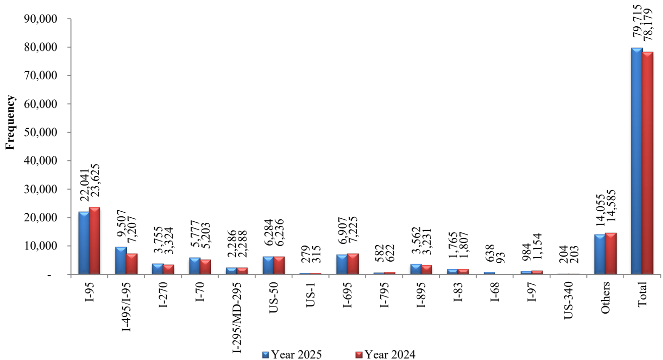
Figure 3.2 Distributions of Incidents/Disabled Vehicles by Road in 2025 and 2024
