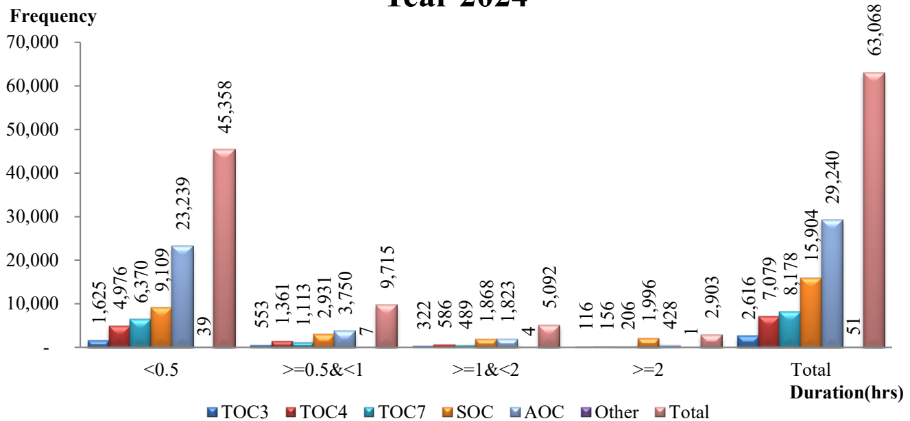
Figure 3.20 Comparisons of Incidents/Disabled Vehicles Distributions by Duration (hrs) and Operation Center
