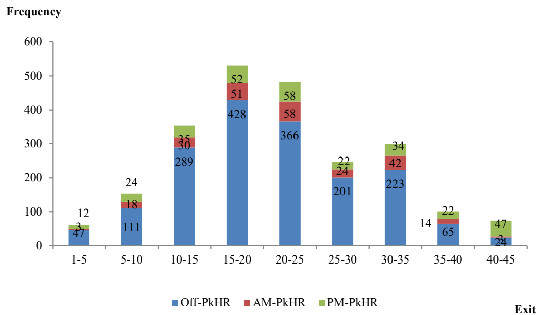
Figure A.8 Distributions of Disabled Vehicles by Time of Day on I-695 in Year 2025
