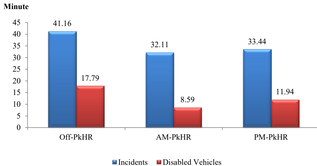
Figure A.15 Distributions of Incident Duration by Time of Day on I/MD-295 in Year 2025
