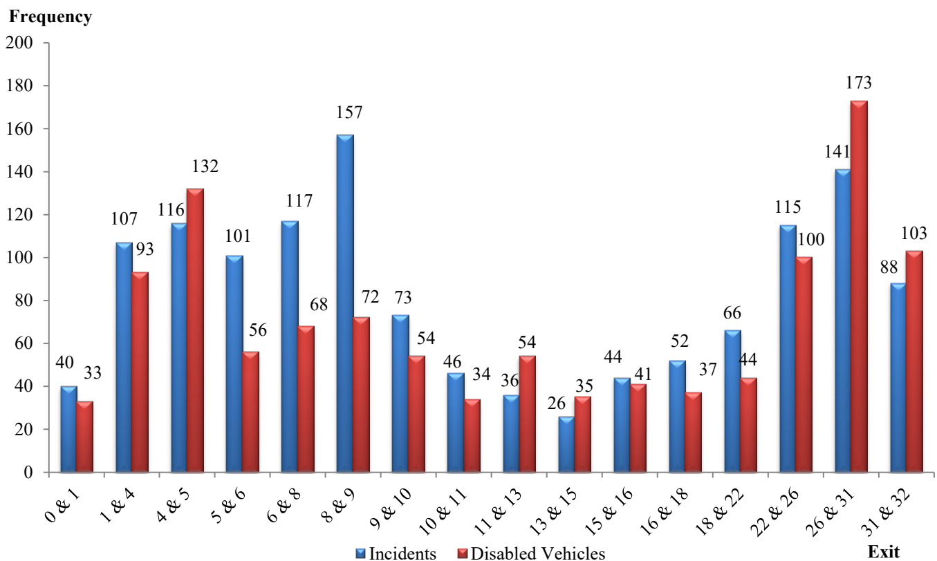
Figure 3.12 Distributions of Incidents/Disabled Vehicles by Location on I-270
