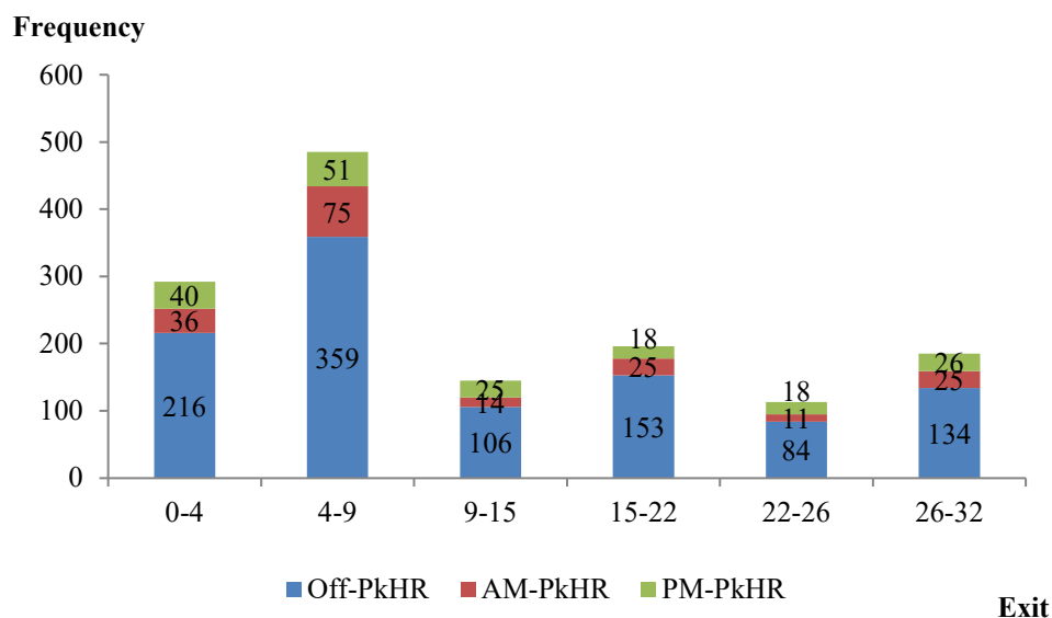
Figure A.5 Distributions of Incidents by Time of Day on I-270 in Year 2025
