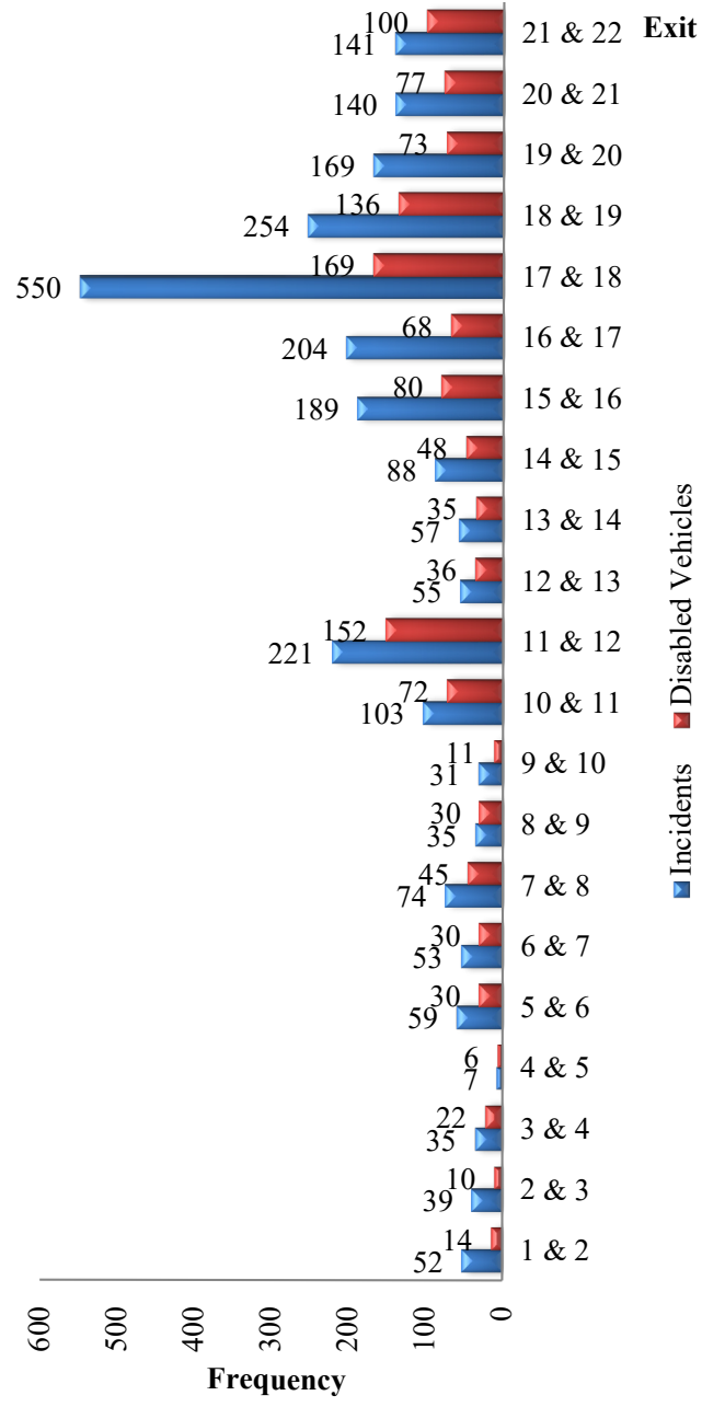
Figure 3.6 Distribution of Incidents/Disabled Vehicles by Location on I-695
