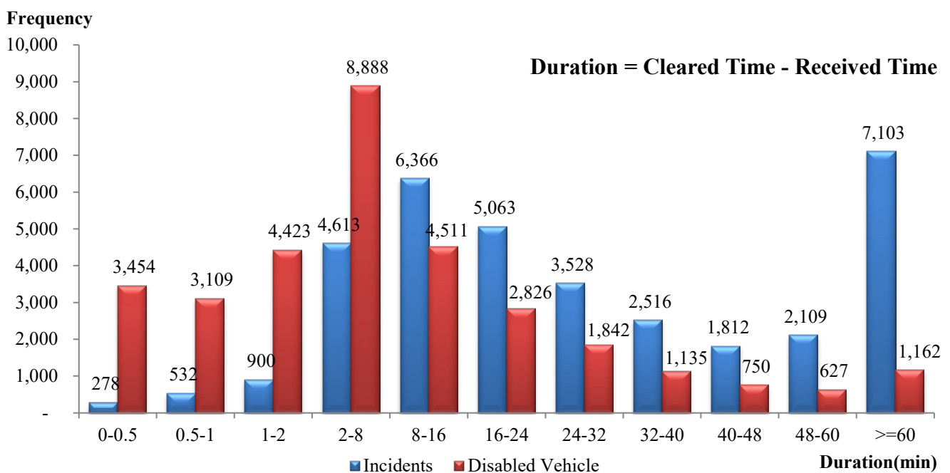
Figure 3.19 Distributions of Incidents/Disabled Vehicles by Duration in 2025
