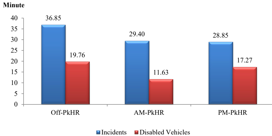
Figure A.14 Distributions of Incident Duration by Time of Day on I-695 in Year 2025
